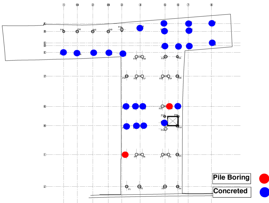
Figure 01 – Graphical representation of pile progress
